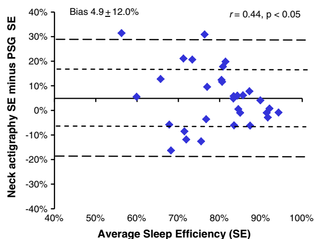
Fig. 2 Bland–Altman plot comparing sleep efficiency between PSG and neck actigraphy
